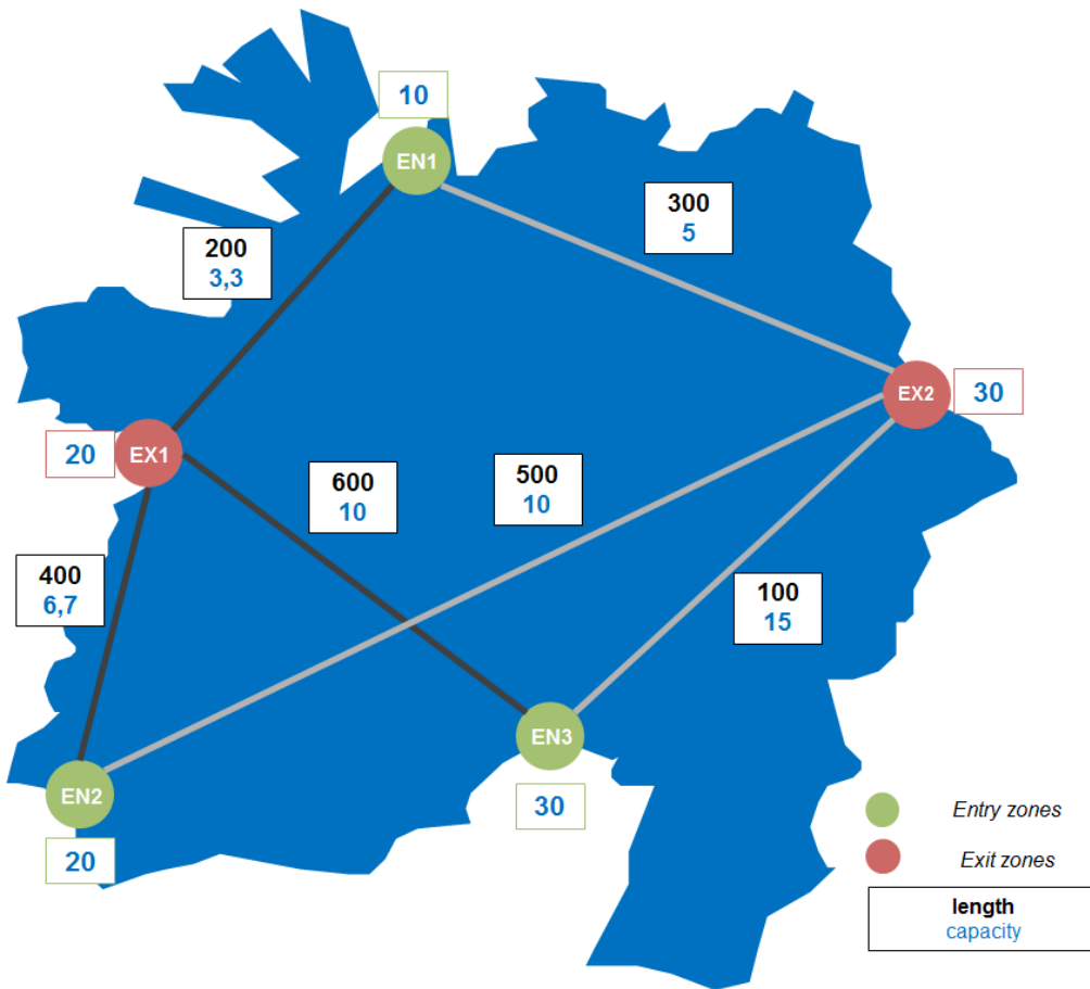
Figure 8: Network Topology
